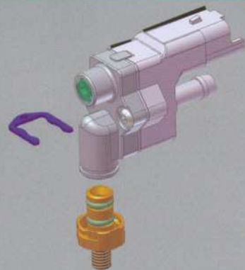
Manifold Version
